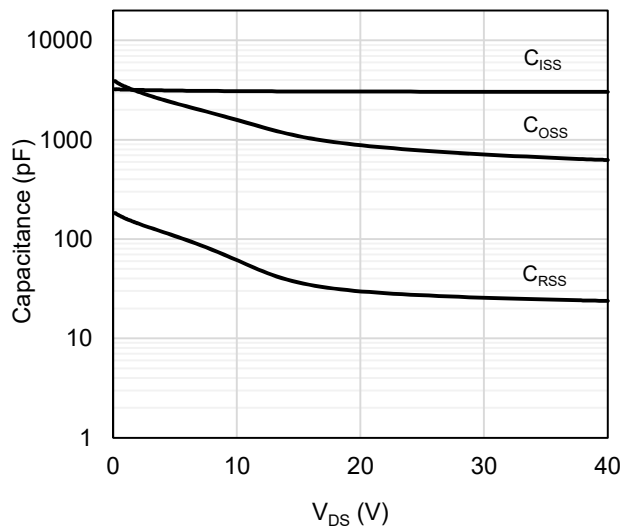
Figure 9: Capacitance Characteristics
