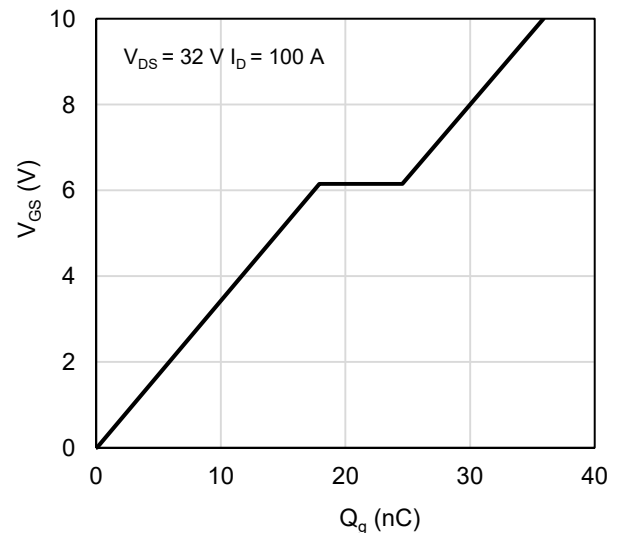
Figure 10: Gate-Charge Characteristics
